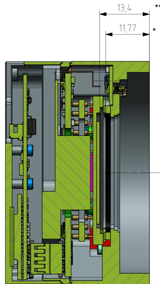
SECTION C-C
