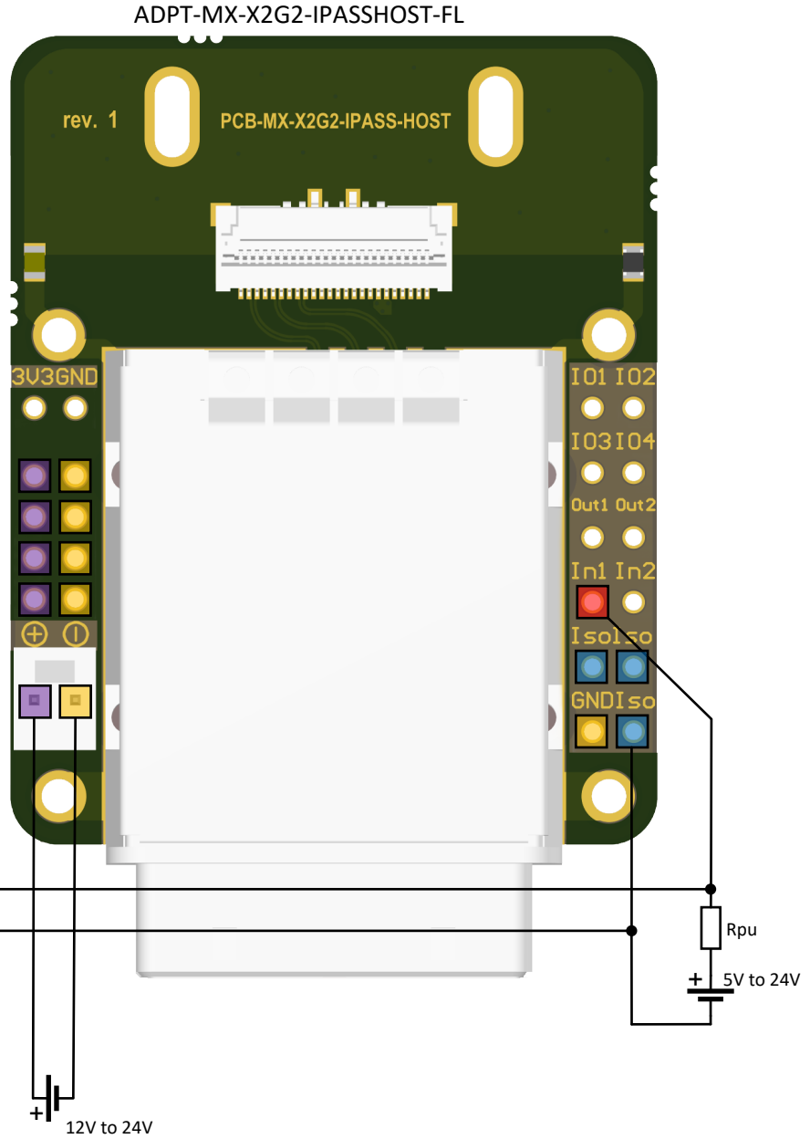
SLAVE Camera
