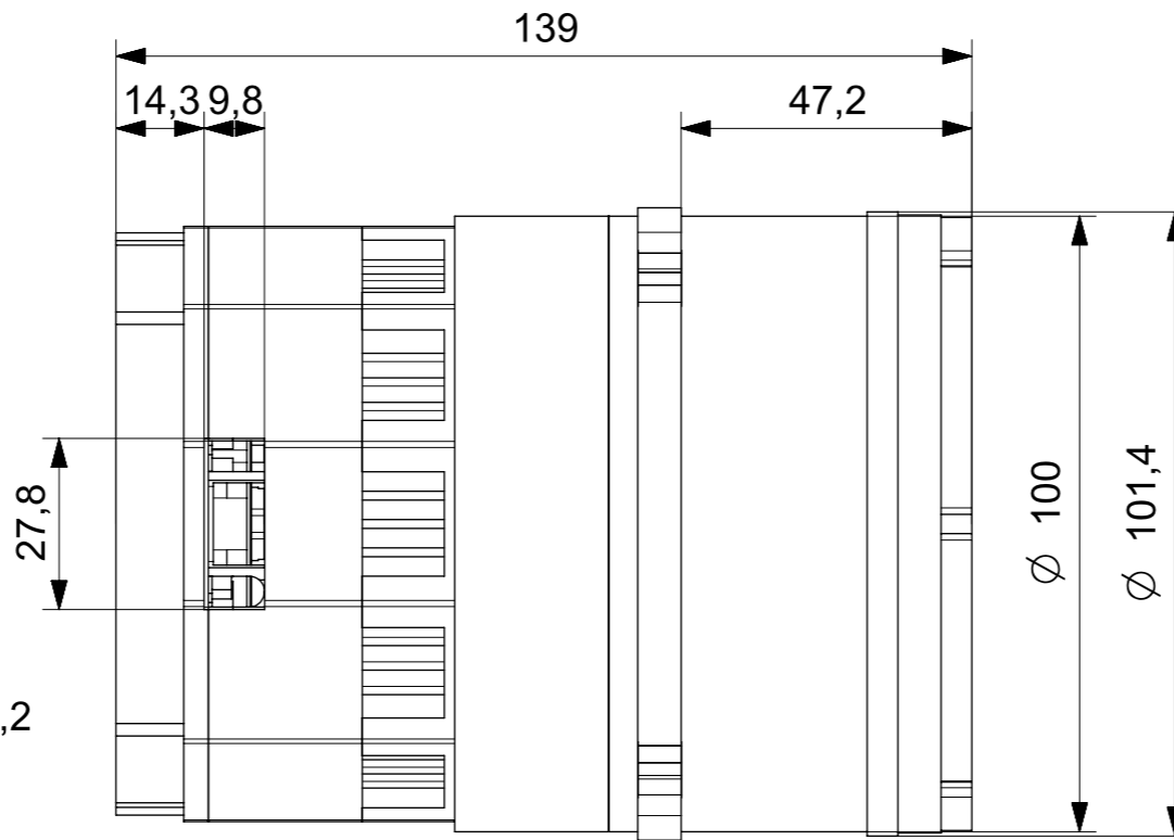
VIEW B SCALE 3:4
