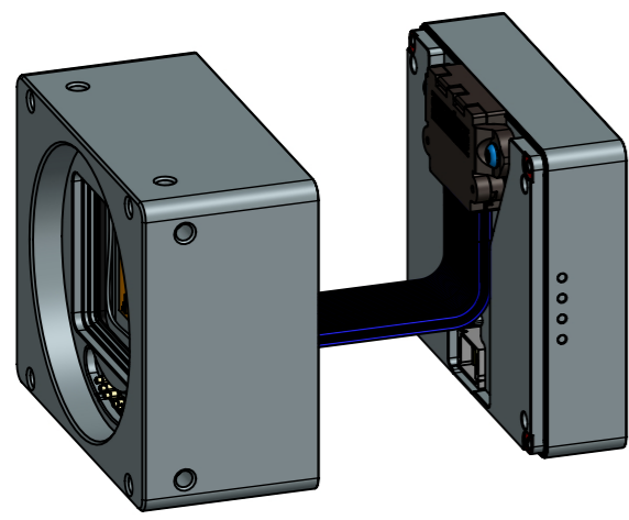
Cameras front and rear sub-assembly detached option
