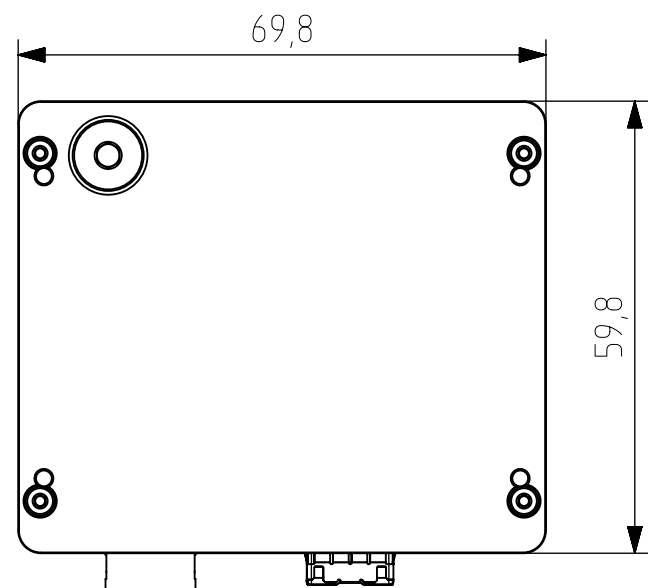
X4G3 SFF accessory module
