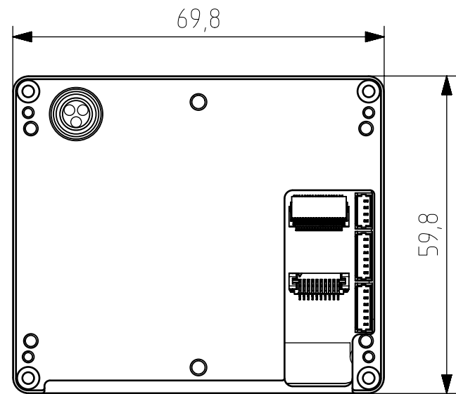
X4G3 Firefly rear module
