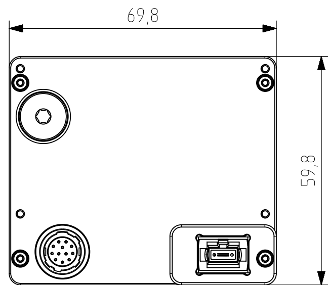
X4G3 MTP accessory module
